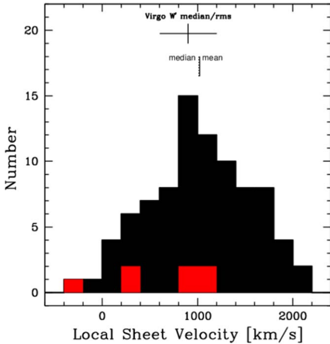
Figure 8. Histogram of velocities (R. B. Tully et al. 2009; E. Kourkchi & R. B. Tully 2017) of the 85 galaxies in the HST SBF sample in black and the seven galaxies in the JWST TRGB sample in red. The mean and median velocities are almost the same: 1023 km s -1 and 1013 km s -1 , respectively, in the Local Sheet reference frame. The mean and variance of velocities in the Virgo W' group are shown at the top of the figure.
