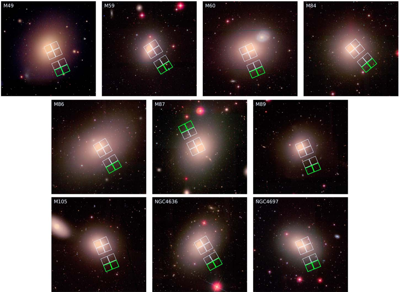
Figure 3. Footprints of our JWST/NIRCam observations, overlaid on 15' \times 15' gri imaging from the Sloan Digital Sky Survey. NIRCam chips in green are those used for our TRGB analysis.
