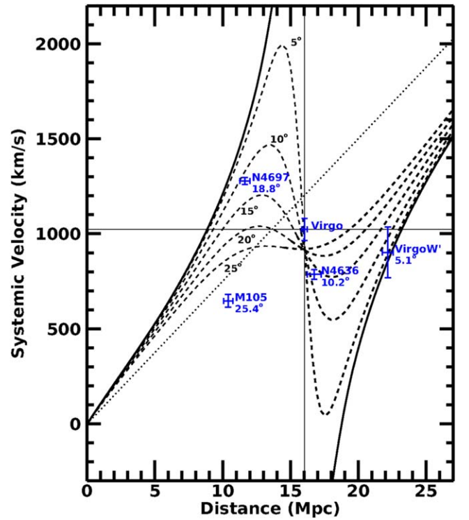
Figure 9. Distances and velocities of systems near the Virgo Cluster discussed in the text superimposed on a model Virgo infall pattern. The name and angular separation from M87 are provided alongside each distance–velocity point. The solid line shows the pattern in the Virgo Cluster direction, and the dashed triple-value curves depict the velocity pattern along lines of sight with angular separations from M87 as labeled on each curve. The diagonal dotted line is for a pure Hubble flow centered on the Local Group.
