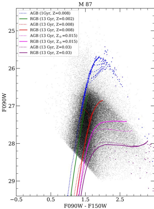
Figure 6. CMD of M87 with the PARSEC isochrones overplotted. The isochrones were shifted according to the distances measured in this paper and Galactic extinction from E. F. Schlafly & D. P. Finkbeiner (2011). The models demonstrate that the downward slope of the TRGB is expected for uniformly old, increasingly metal-rich populations.
