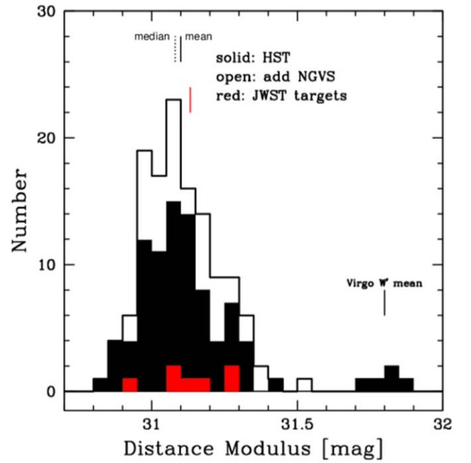
Figure 1. Histogram of distances to members of the Virgo Cluster and background Virgo W' Cluster from the HST ACS and NGVS SBF surveys. The filled histogram is from ACS alone, and the open histogram is from the sum of the two studies. The filled red histogram shows the values in these surveys associated with the JWST targets discussed in this paper. The median and mean distance modulus values for the Virgo ensemble are 31.10 and 31.08 mag, respectively. The mean value for the seven JWST cases is 31.13 mag. The median distance modulus value for Virgo W' is 31.80 mag.
