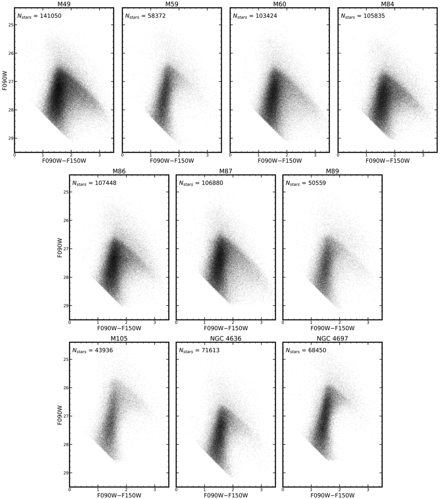
Figure 5. CMDs for each of the 10 galaxies presented in this paper. The CMDs for each of the two chips are combined and displayed for each target, and the total number of stars is displayed in the top left. Only stars in the range 0.50 \text{ mag} \leq F090W - F150W \leq 1.75 \text{ mag} were used for the determination of the TRGB due to the downward sloping of the TRGB at higher metallicities and redder colors (G. S. Anand et al. 2024a).
